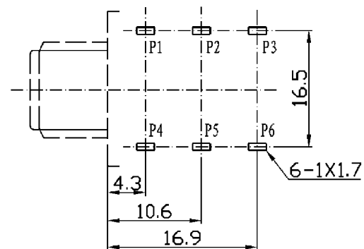
Dimensions of PC board holes (Commend)
