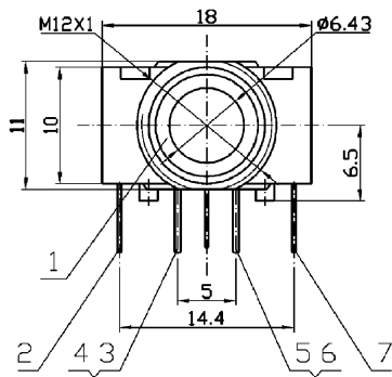
Dimensions of PC board holes (Commend)
