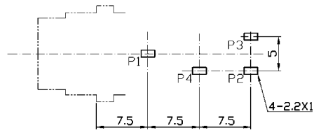
Dimensions of PC board holes (Commend)
