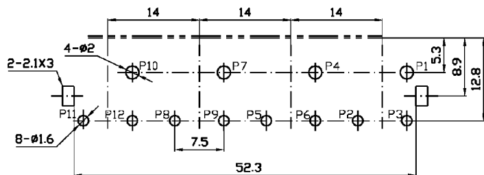
Dimensions of PC board holes (Commend)
