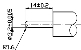
Gauge Plug
