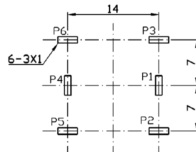
Dimensions of PC board holes (Commend)
