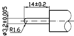
Gauge Plug
