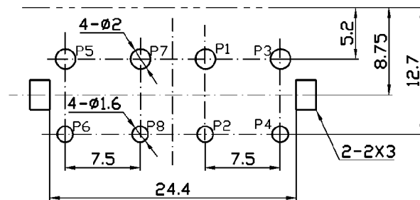
Dimensions of PC board holes (commend)
