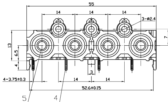
Dimensions of PC board holes (Commend)
