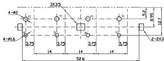
Dimensions of PC board holes (Commend)
