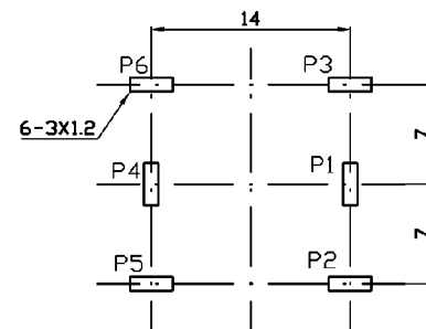
Dimensions of PC board holes (Commend)
