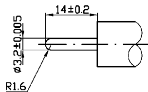
Gauge Plug
