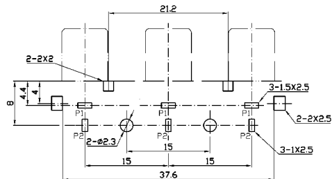
Dimensions of PC board holes (Commend)
