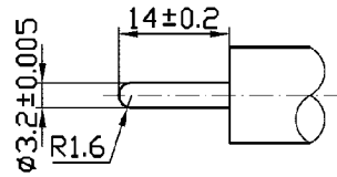
Gauge Plug
