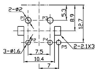
Dimensions of PC board holes (Commend) Bottom View (t=1.6mm) \odot
