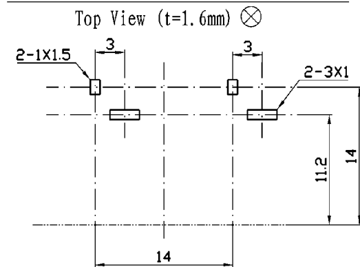
Dimensions of PC board holes (Commend)
