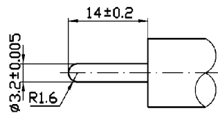
Gauge Plug
