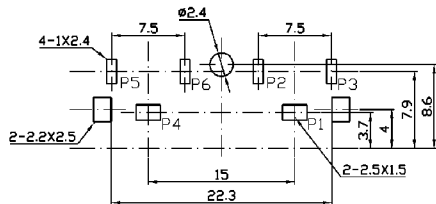
Dimensions of PC board holes (Comment)
