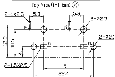
Dimensions of PC board holes (Commend)
