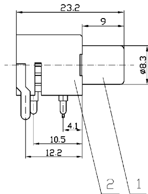
Gauge Plug
