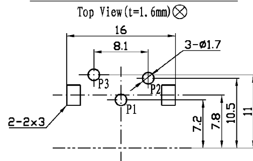
Dimensions of PC board holes (Commend)
