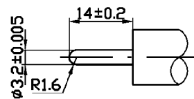
Gauge Plug
