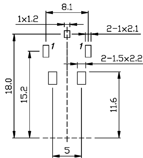
P.C.B LAYOUT( \pm 0.1 ) (BOTTOM VIEW)
