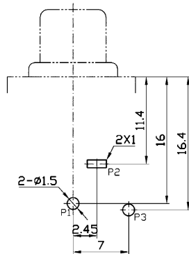
Dimensions of PC board holes (Commend)
