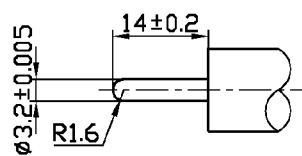
Gauge Plug
