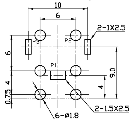
Dimensions of PC board holes (Commend)
