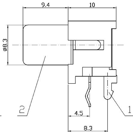
Dimensions of PC board holes (Commend)
