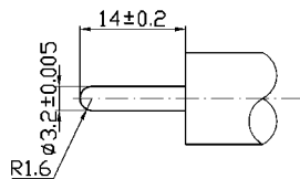
Gauge Plug
