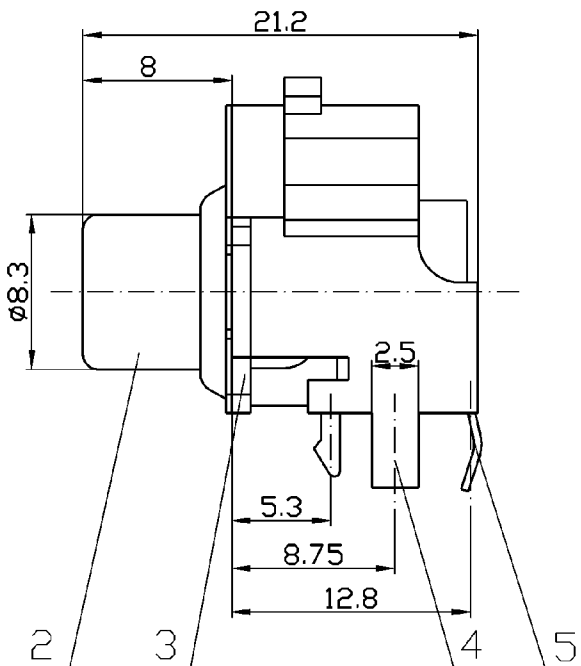
Gauge Plug
