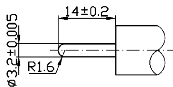
Gauge Plug
