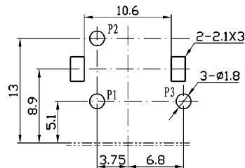
Dimensions of PC board hole (Commend)
