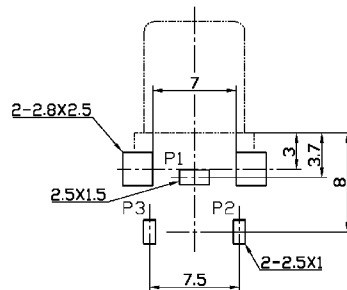
Dimensions of PC board holes (Comment)
