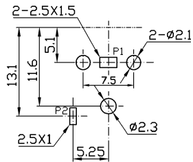
Dimensions of PC board holes (commend)
