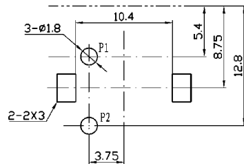
Dimensions of PC board holes (Commend) Bottom View (t=1.6mm) \odot
