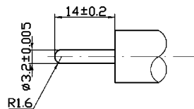
Gauge Plug
