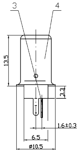
Gauge Plug
