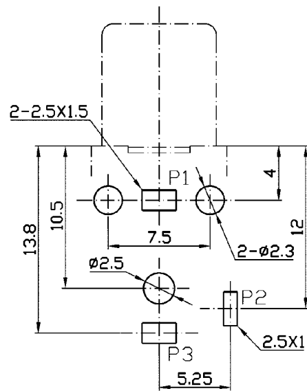
Dimensions of PC board holes (Commend)
