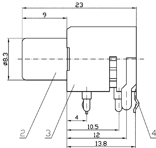
Gauge Plug
