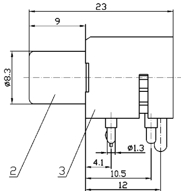
Gauge Plug
