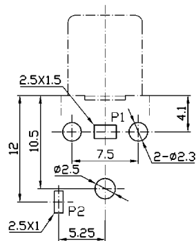
Dimensions of PC board holes (Commend) Bottom View (t=1.6mm) Ⓢ
