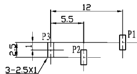
Dimensions of PC board holes (Commend)
