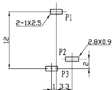
Dimensions of PC board holes (Commend)
