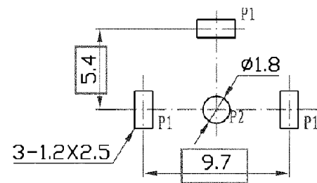
Bottom View (t=1.6mm) Ⓢ
