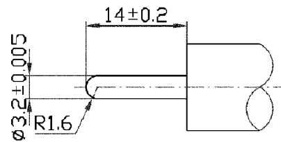
Gauge Plug
