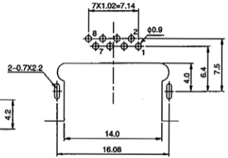
Recommend PCB Layout Jack Top View
