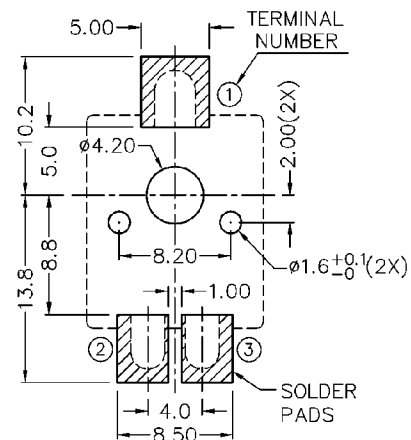
RECOMMENDED SOLDER PAD LAYOUT (TOP VIEW)
