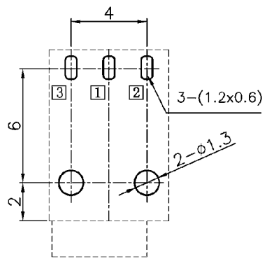
RECOMMENDED P. C. B. LAYOUT UNSPECIFIED TOLERANCE: \pm 0.05 (COPPER-SIDED VIEW)
