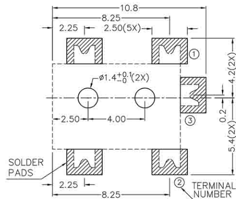
RECOMMENDED SOLDER PAD LAYOUT (TOP VIEW)
