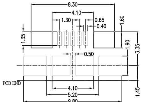
DIMENSIONS OF PC BOARD HOLES (COMMEND) TOP VIEW ⊗
