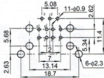
Recommend PCB Layout Jack Top View
