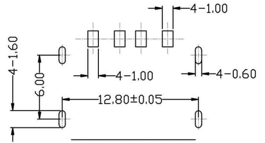
FRONT EDGE OF CONNECTOR PCB LAYOUT (T=1.40mm)
