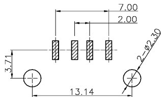
RECOMMENDED P.C.B. PATTERN LAYOUT
