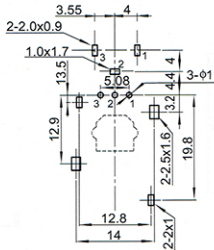
Recommend PCB Layout Jack Top View
