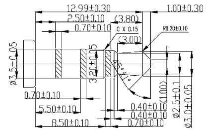
#3.50mm 4 POLE PLUG DETAIL DRAWING
