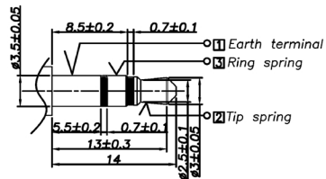
Matching Plug
