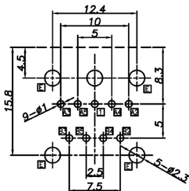
P.C.B Layout (Copper-sided view)
