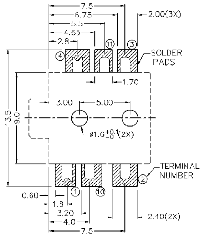
RECOMMENDED SOLDER PAD LAYOUT
