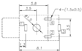
P. C. B Layout (Copper-sided view)
