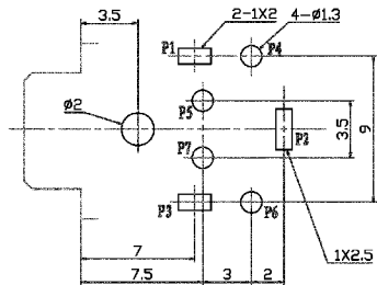
Dimensions of PC board holes (Commend) Bottom View (t=1.6mm)
