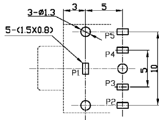
Dimensions of PC board holes (Commend) Bottom View \odot (t=1.6)
