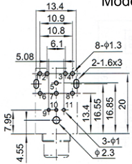
Recommend PCB Layout Jack Top View
