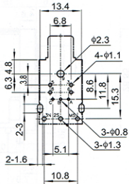
Recommend PCB Layout Jack Top View
