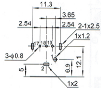
Recommend PCB Layout Jack Top View
