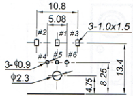
Recommend PCB Layout Jack Top View
