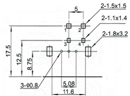
Recommend PCB Layout Jack Top View
